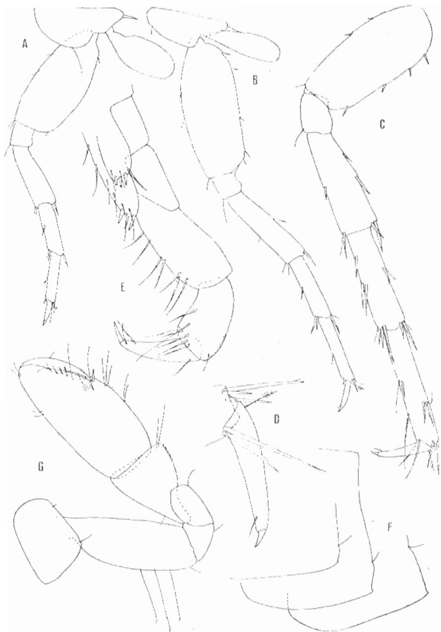
Fig. 3. Bogidiella (Bogidiella) calicali , n. sp., Castelsardo, female 2.5 mm: A = pereopod 5; B = pereopod 6; C-D = pereopod 7; E = maxilliped; F = epimeral plates 1-3; G = gnathopod 2, male 2.5 mm from Rio di Quirra.
