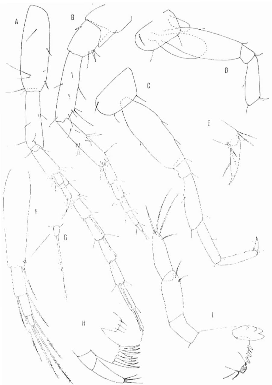
Fig. 1. Bogidiella (Bogidiella) calicali , n. sp., Castelsardo, female 2.5 mm: A = antenna 1; B = antenna 2; C = pereopod 3; D-E = pereopod 4; F-G = pleopod 2; H = maxilla 1; I = mandible.
