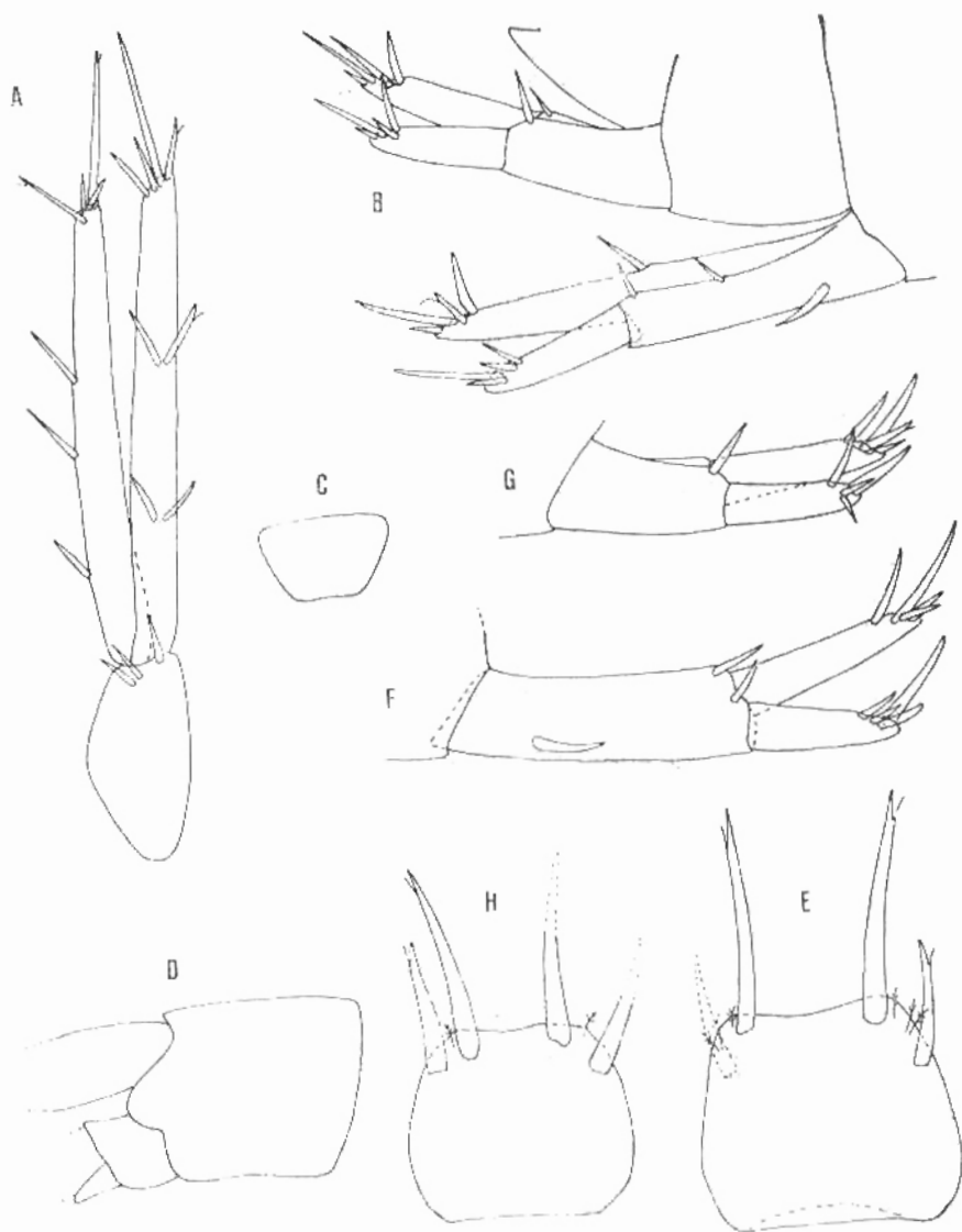
Fig. 4. Bogidiella (Bogidiella) calicali , n. sp., Río di Quirra, male 2.5 mm: A = uropod 3; B = uropods 1-2; C = labrum; D = head, female 2.5 mm; E = telson, female 2.5 mm; F-G = uropods 1-2, female 2.5 mm from Castelsardo; H = telson, female 2.5 mm from Castelsardo.
